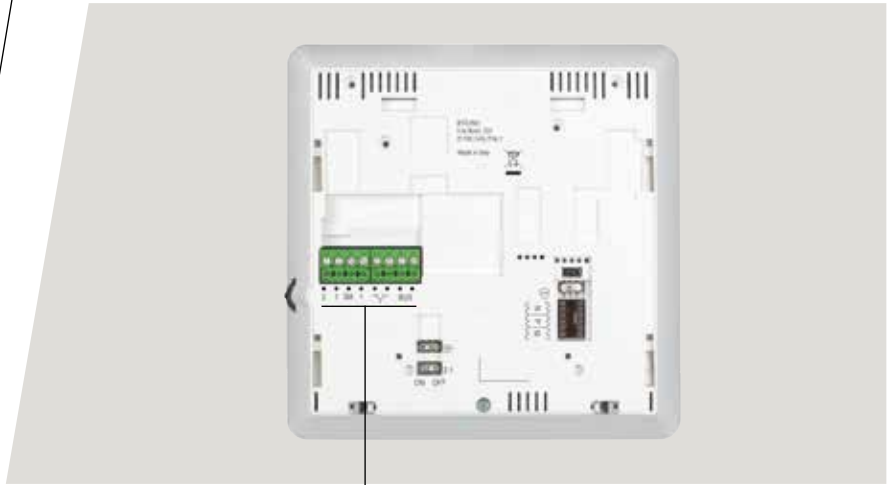
BTicino 2 wires video indoor units have standard plug-in SCS BUS clamps: maximum simplicity.
